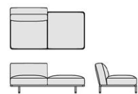
MS_60L - MS_60LP cm. 180x100x38/70h inch 70 3 / 4 x39 1 / 4 x15 1 / 2 "
