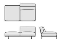
MS_60R - MS_60RP cm. 180x100x38/70h inch 70 3 / 4 x39 1 / 4 x15 1 / 2 "
