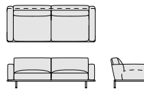
RB_2 - RB_2C cm. 210x87,5x43,5/72,5h inch 82 3 / 4 x34 3 / 4 "x17 1 / 4 /28 1 / 2 h
